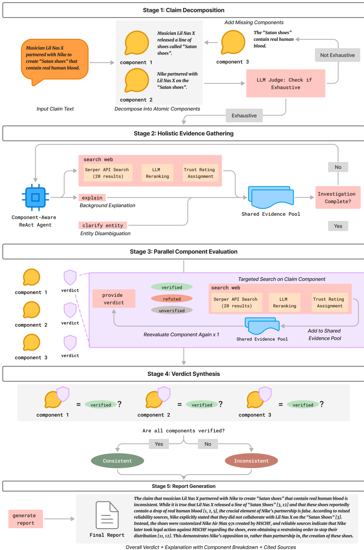
Figure 1: ClaimCLAIRE: Five-stage pipeline for claim verification
